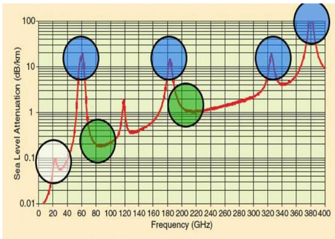
Figure 4 – Atmospheric absorption across mm-wave frequencies in dB/km [3]
